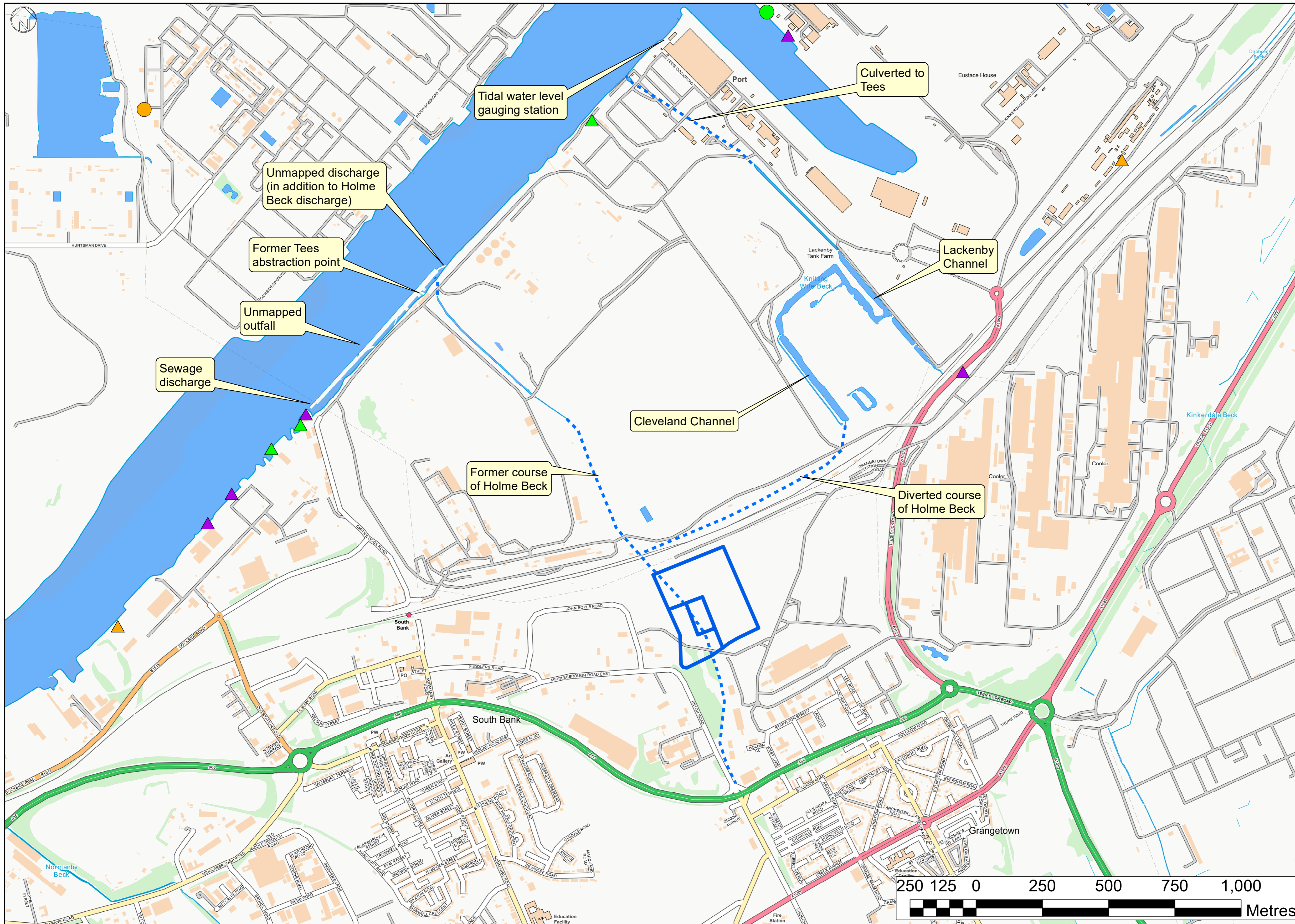
FIGURE 8-1: SITE LOCATION AND HYDROLOGICAL FEATURES 1:7,500 @ A1 / 1:15,000 @ A3
